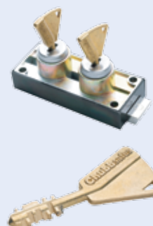
Dual control Lock with 2 key Locks
